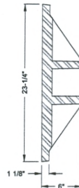
SECTION B - B
