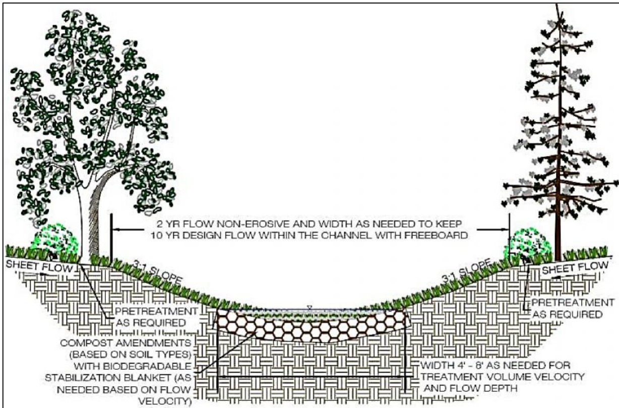
Figure 7A.4: Grass Channel with Compost Amendments - Section
