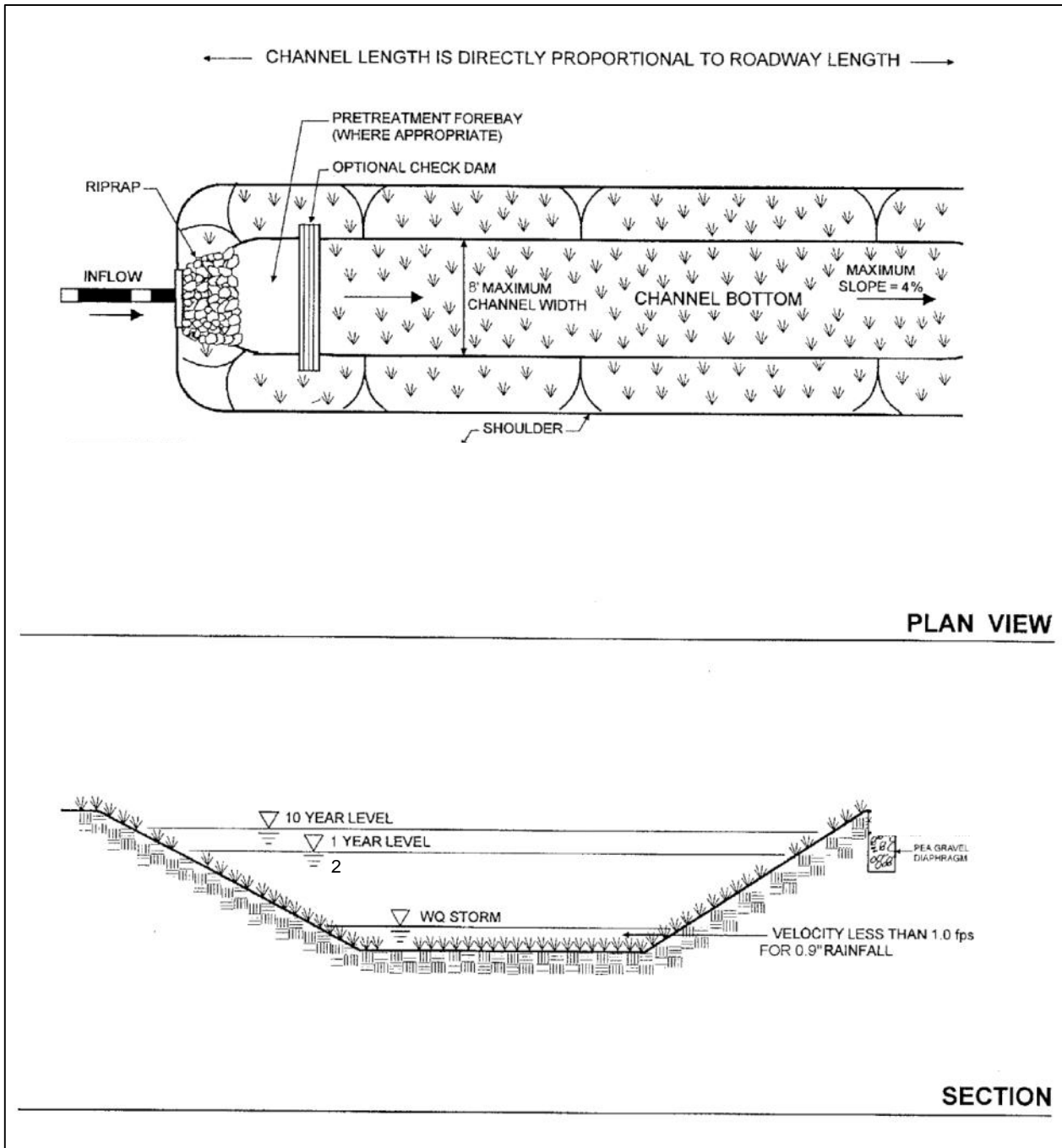
Figure 7A.2. Grass Channel – Typical Plan, Profile and Section (Source: VADCR, 2011, MWS edited 2020)
