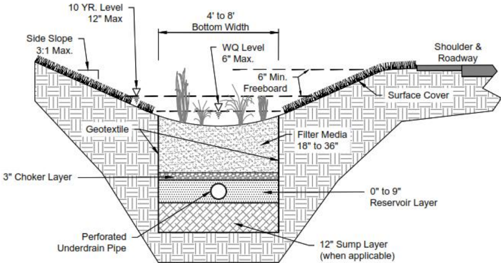
GIP - 05B WATER QUALITY SWALE WITHOUT UNDERDRAIN
