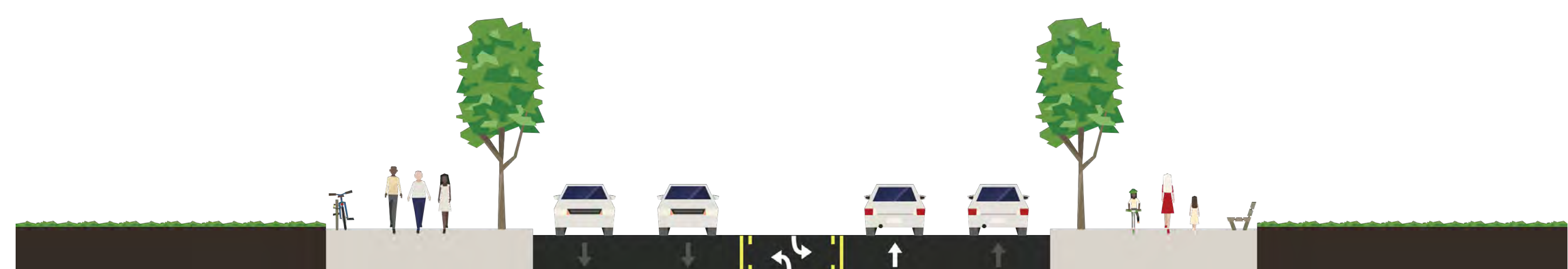
Consolidated Cross-Section - Turn Lane Condition
