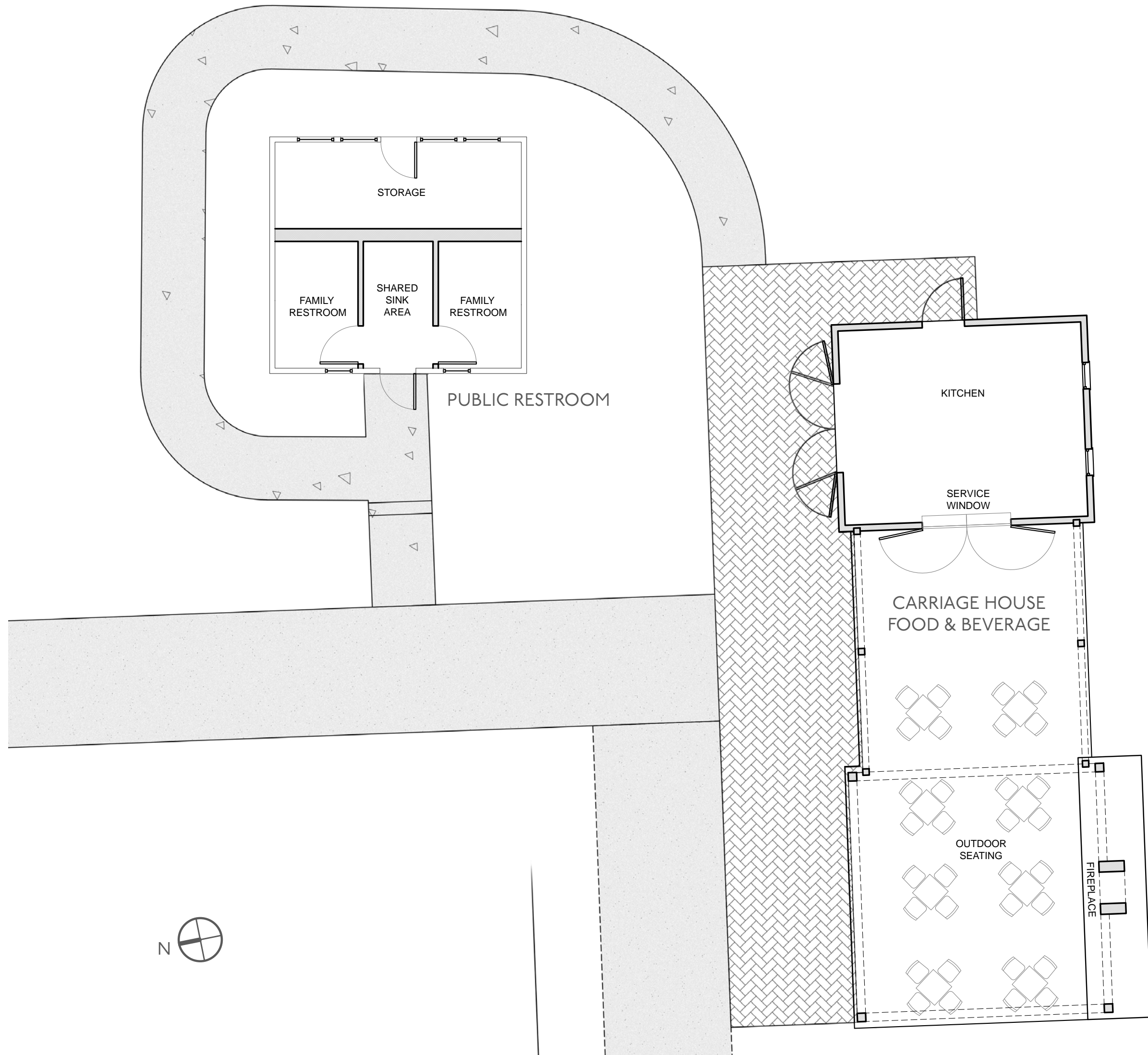
CARRIAGE HOUSE & PUBLIC RESTROOM PLANS
