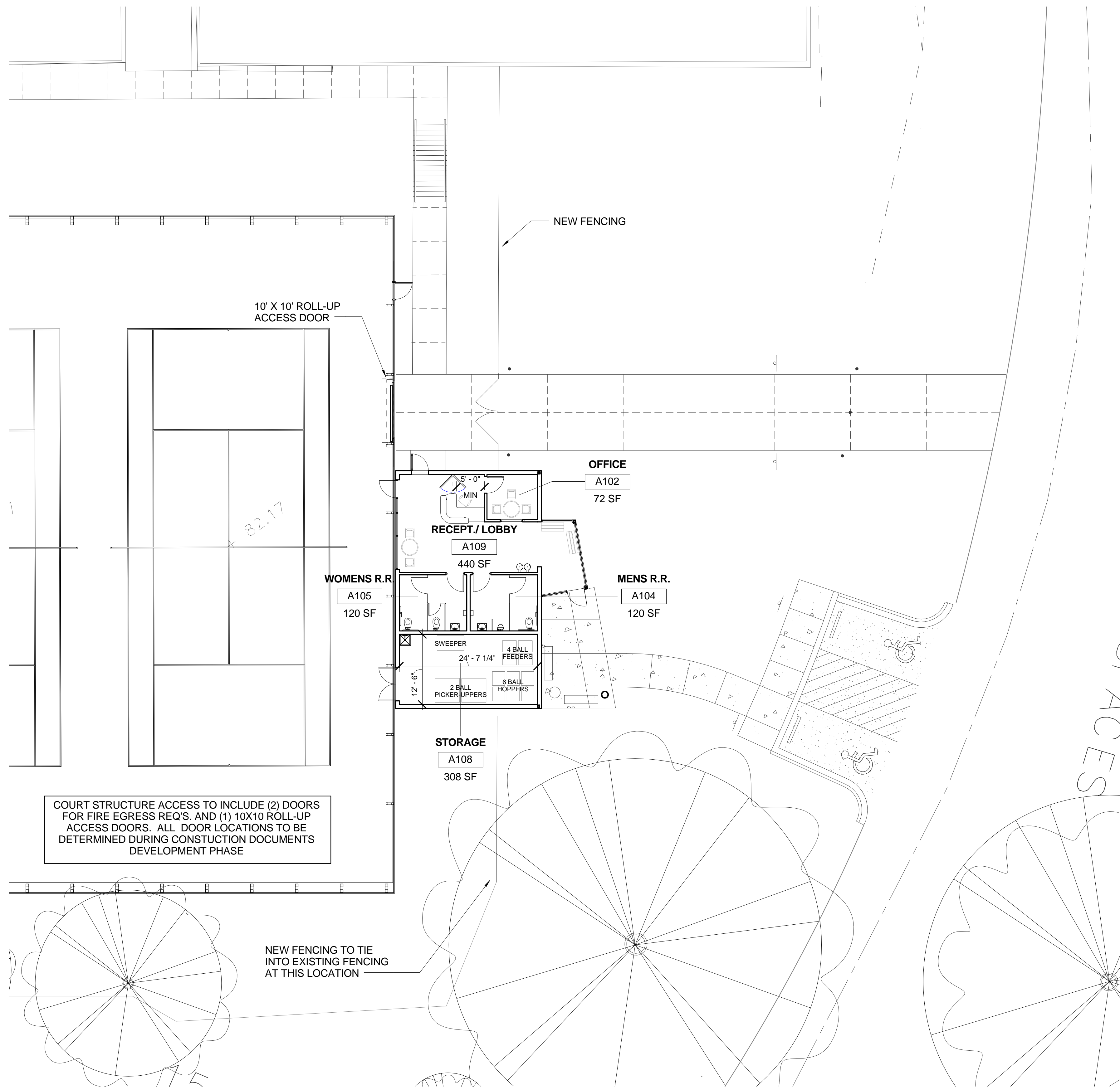
1 FLOOR PLAN - PRESENTATION PLAN 3/32" = 1'-0" BUILDING AREA: 1,175 SF
